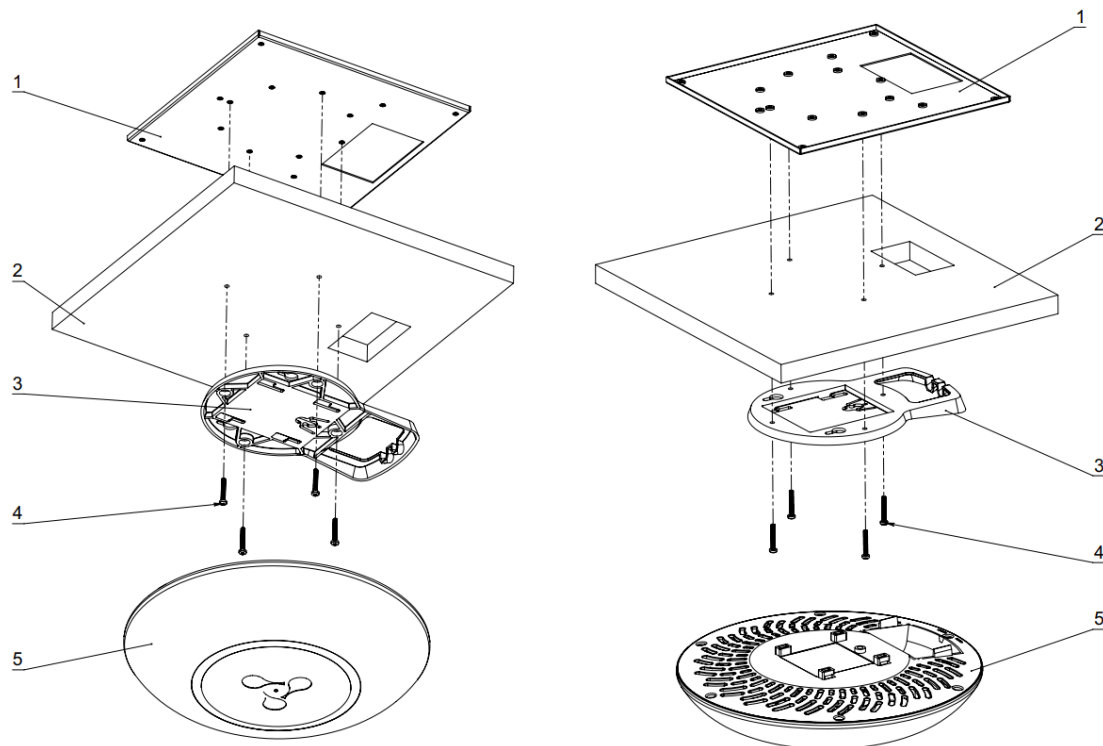
Figure 8 – Mounting on a false ceiling
